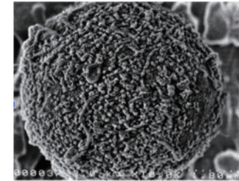
Photo of influenza virus being absorbed by the surface of hydroxyapatite particles (PENTAX)
